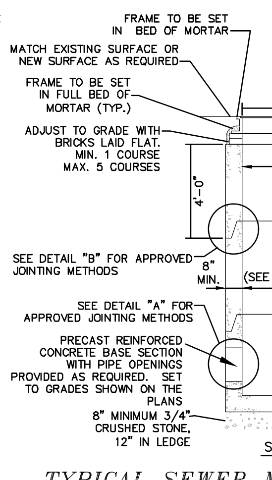
TYPICAL SEWER MANHOLE NOT TO SCALE
