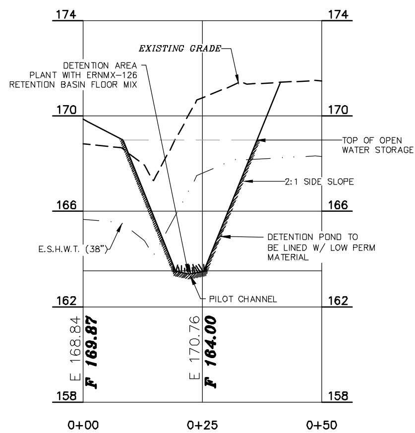
SECTION OF DETENTION POND #102
