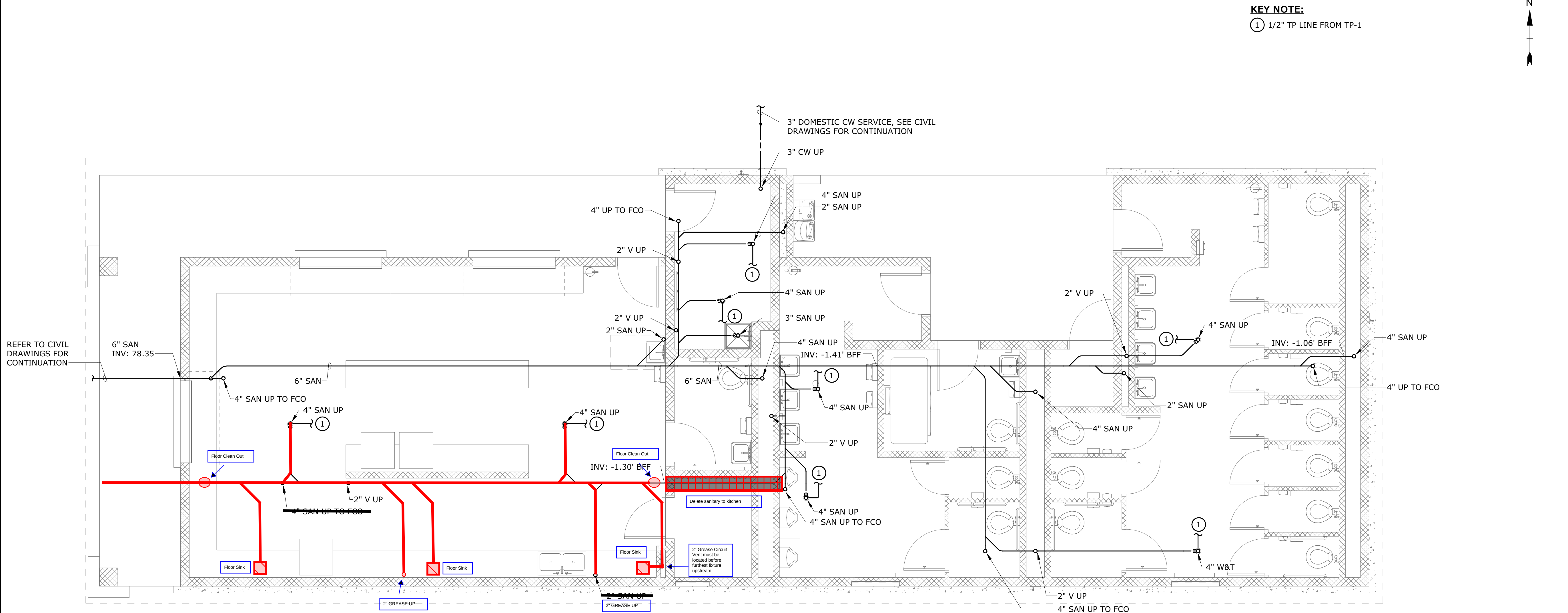
PLUMBING CONCESSIONS BUILDING UNDERGROUND PLAN SCALE: 1/4" = 1'-0"
