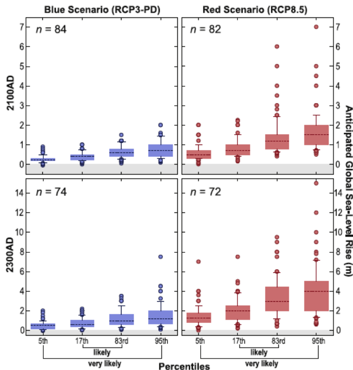
Figure 2.9. Results of expert survey of sea-level rise expectations, from Horton et al (2013).
