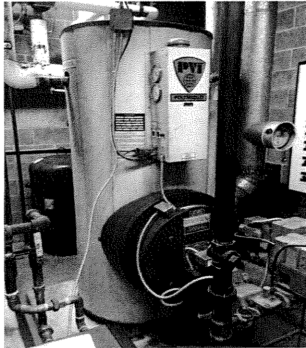
CTC original hot water heater from 1989
