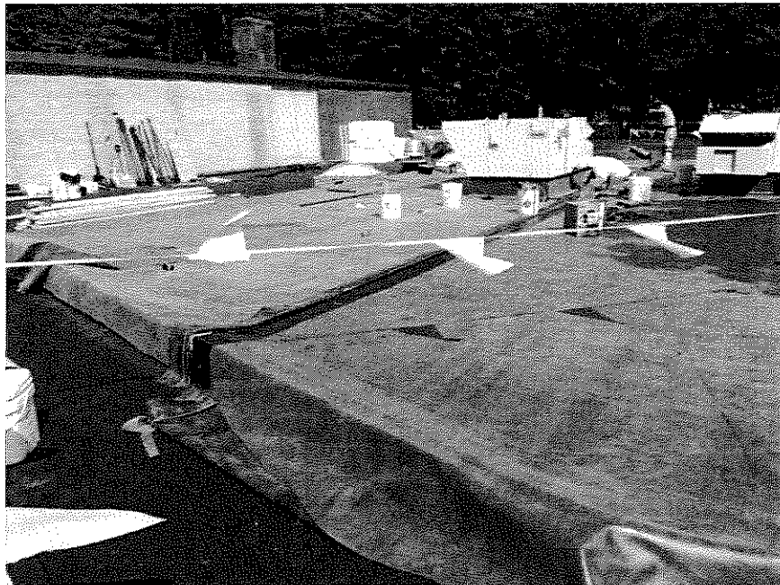
Garrison roof new rubber membrane being applied
