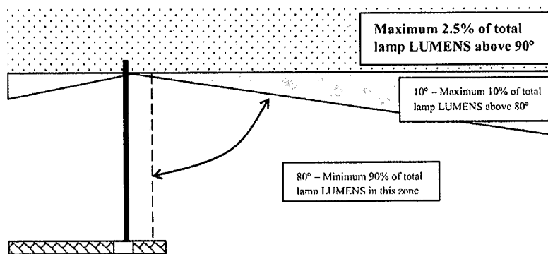
Cutoff fixture as defined by IESNA
